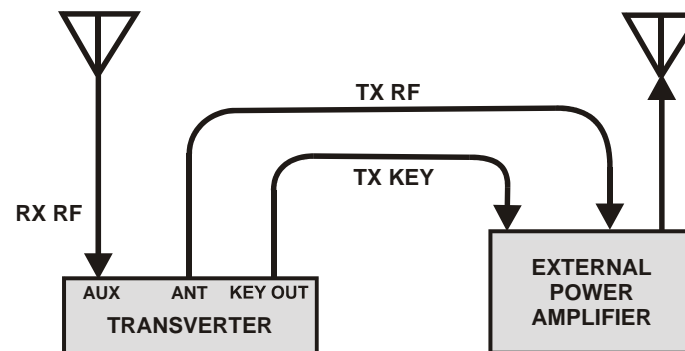
Figure 10. Using an External Power Amplifier.
